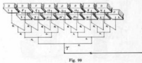
Ernest Skimmer's "wbiffletree" swell engine concept, in which 16 pneumatics move a common trace incrementally
